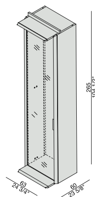
Modulo scarpiera Shoe rack module
