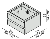
Cassettiera 2 cassetti 63 2 Drawers chest 63
