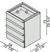
Cassettiera 4 cassetti 63 4 Drawers chest 63
