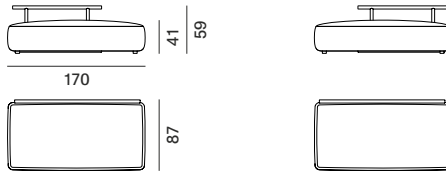
module seat L with back structure L110 L/R
