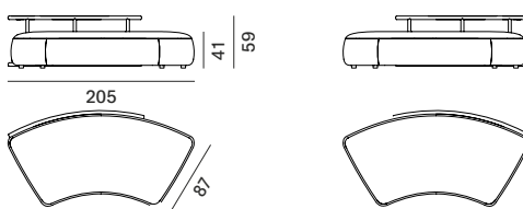
curved module seat M with back structure L155 L/R
