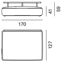
module seat L deep with back structure L155
