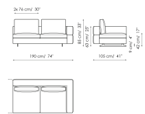
End section sofa 190
