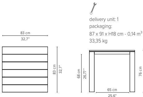
04070 - Dining table 83 x 83 cm
