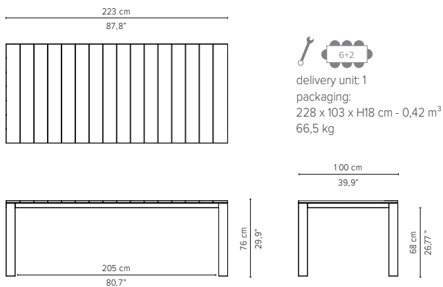
04052 - Dining table 223 x 100 cm
