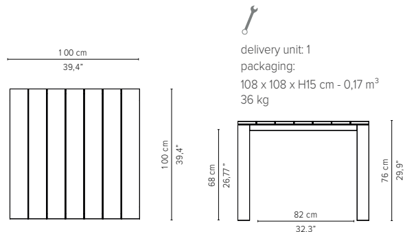
04073 - Dining table 100 x 100 cm
