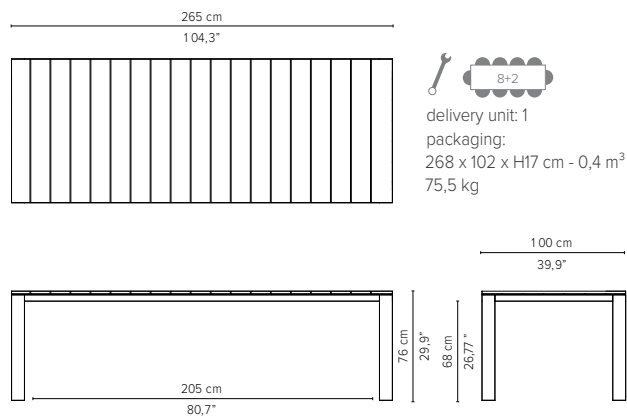
04053 - Dining table 265 x 100 cm
