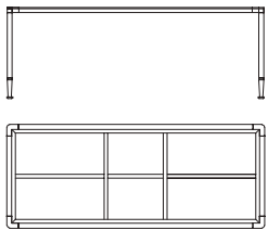
C 87004 Tavolo rettangolare in acciaio, 8 doghe Rectangular table in steel, 8 slats cm 205 x 82 x h 73 in 80 3/4 x 32 1/4 x h 28 3/4
