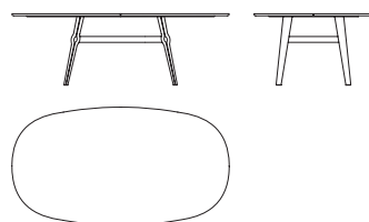
70401 Piano in marmo Marble top cm 220 x 120,5 x h 72 in 86 5 / 8 x 47 1 / 2 x h 28 3 / 8
