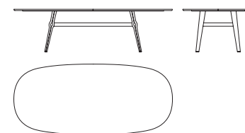
70406 Piano in marmo Marble top cm 270 x 120,5 x h 72 in 106 1 / 4 x 47 1 / 2 x h 28 3 / 8
