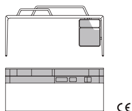
73041 Scrivania con multipresa e cassetiera destra con due alzate e LED Writing desk with multi-socket and right chest of drawers with two upper sections and LED cm 180 x 81 x h 92.2 in 70 7/8 x 31 7/8 x h 36 1/4
