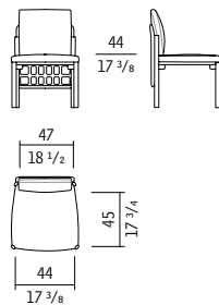
Sedia / Chair / Stuhl / Fauteuil cm 55 x 58 x h 80 in 21 3/8 x 22 7/8 x h 31 1/2
