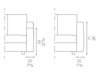
freestanding corner 90°
