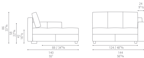
corner 90°
