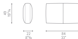
back cushion 84
