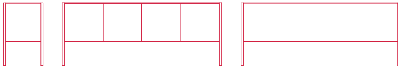
low unit 4 DOORS L200 D50 H80 real dimensions L199.5 D50 H79.7
